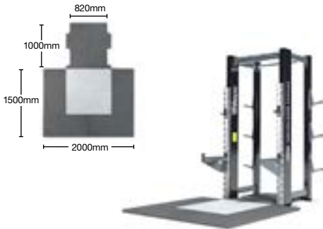
LIFTPLAT6 Integrated Lift Zone - Double Bolted Leg
