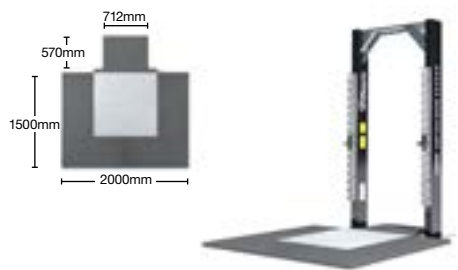
LIFTPLAT8 Integrated Lift Zone - MONO Bolted Leg
